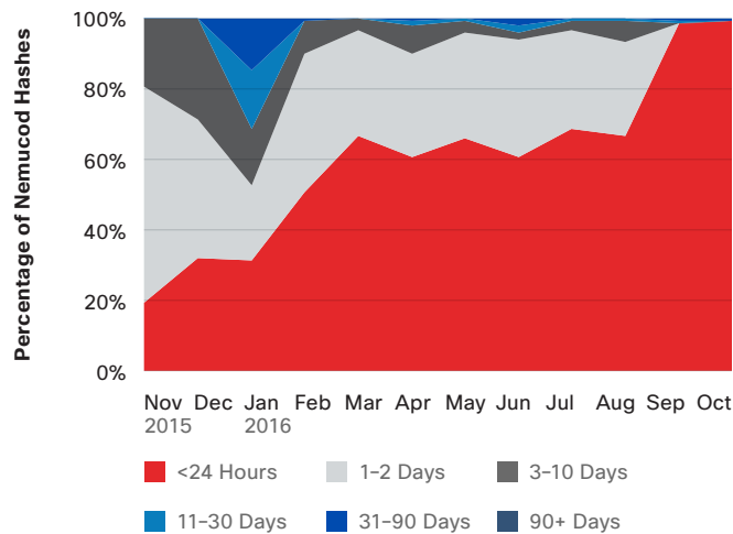
Figure 134 Hash Ages for the Nemucod Malware Family Per Month
