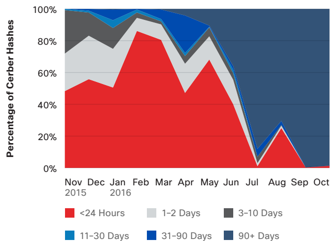
Figure 132 Hash Ages for the Cerber Malware Family and Percent of Total Hash Volume Observed Per Month
