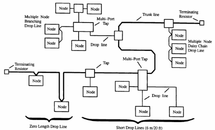
Figure 2 DeviceNet Topology Options
