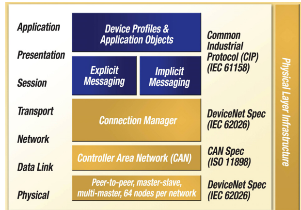
Figure 1 DeviceNet Adaptation of CIP
