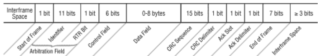
Figure 6 CAN Data Frame Format
